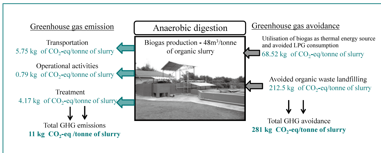
Figure 3 Greenhouse gas emissions and avoidance potential from anaerobic digestion in Muangklang (Note: Dry matter content of the organic slurry is maintained at 8.5% )
